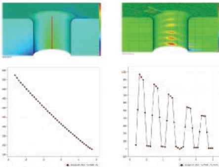
Method of «effective modules of elasticity»
